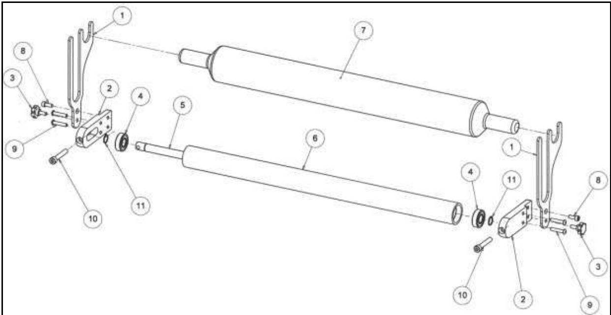
Exploded view 4
