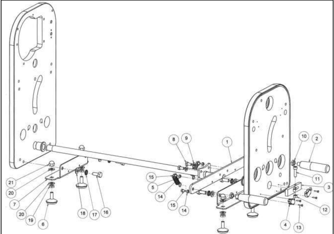
Exploded view 8 (FOR OVER THE COUNTER SFG 500)
