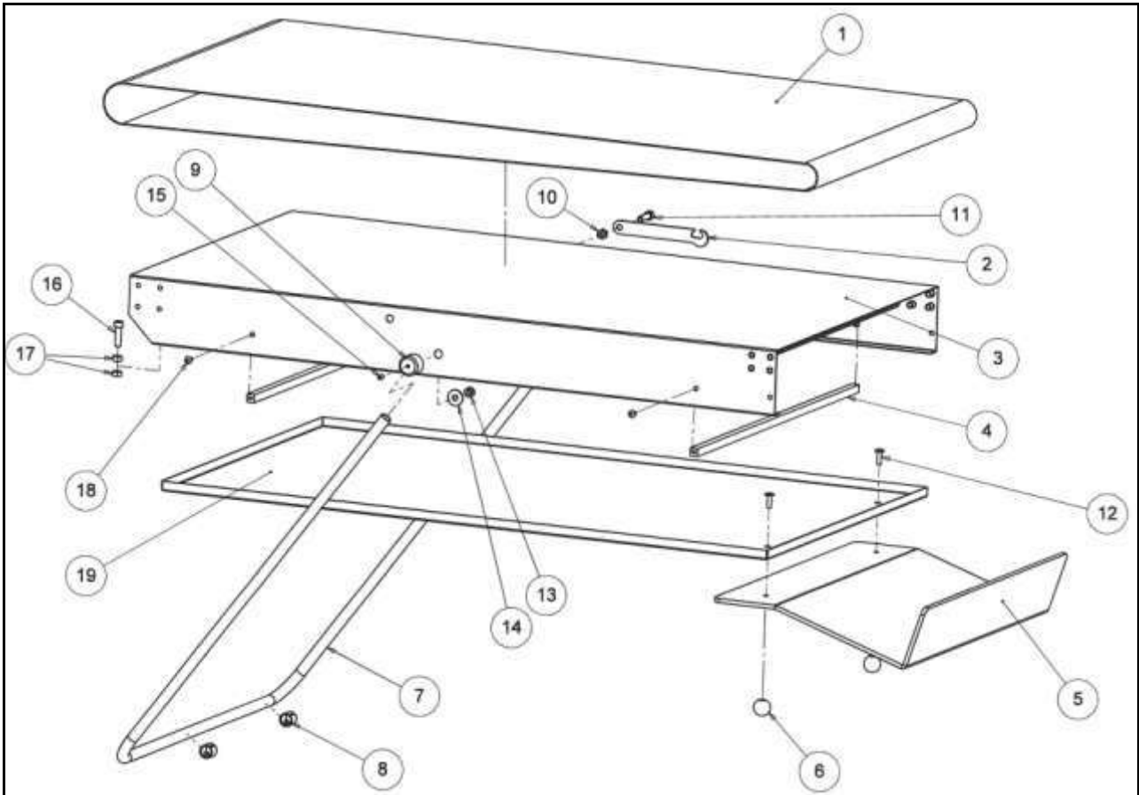
Belt SFG 500 TM Table
