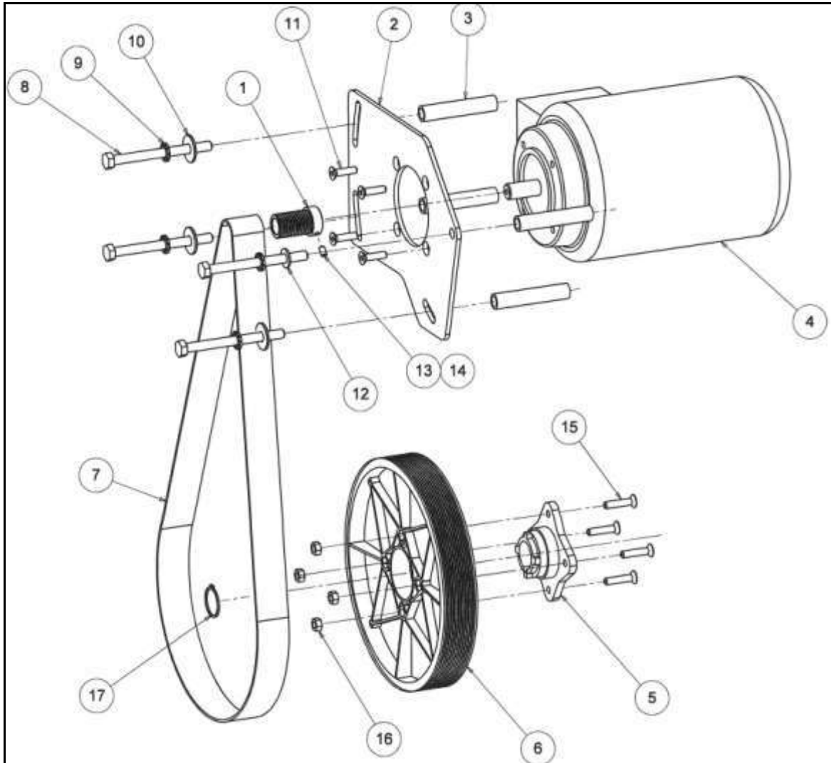
Exploded view 5
