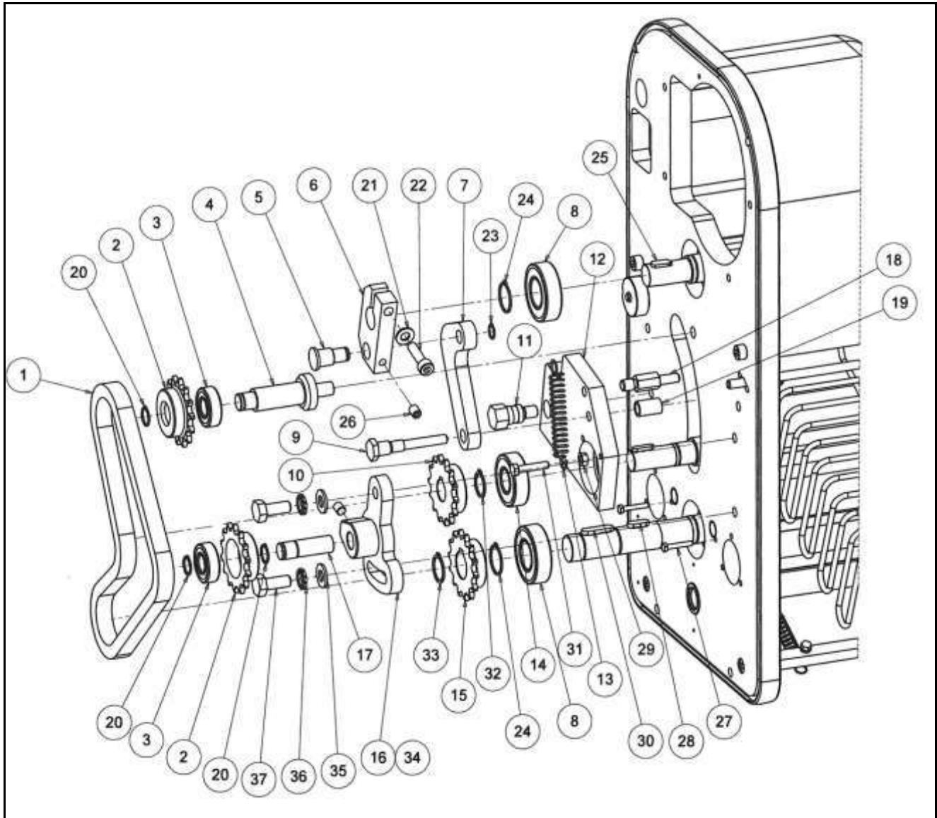
Exploded view 6A
