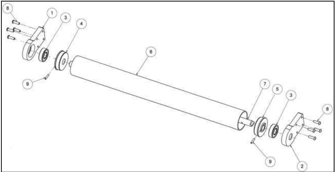
Exploded view 3
