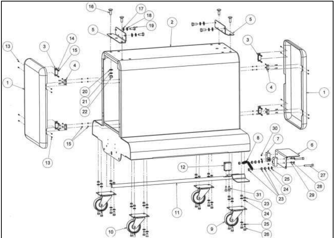
Exploded view 9
