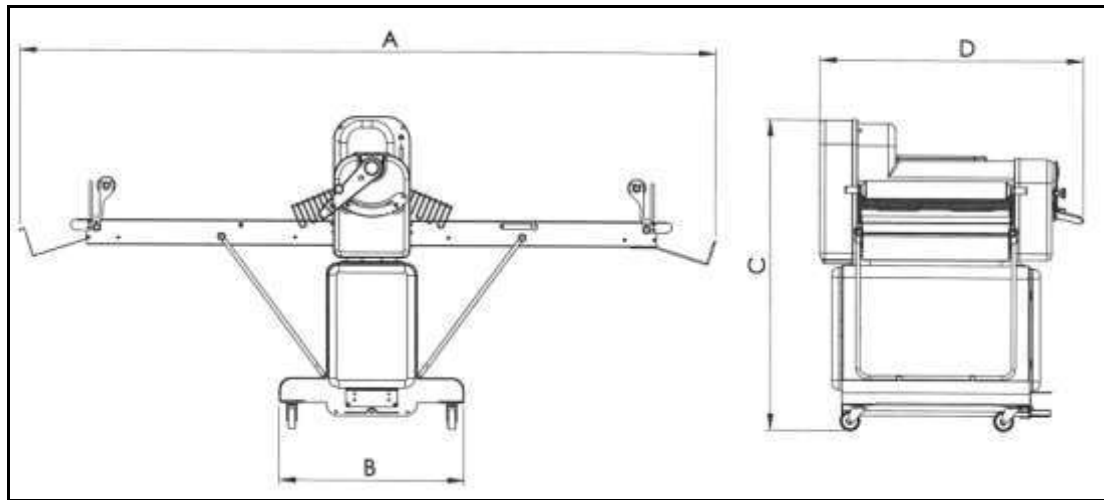
Sheeters 500 T - 500 TM
